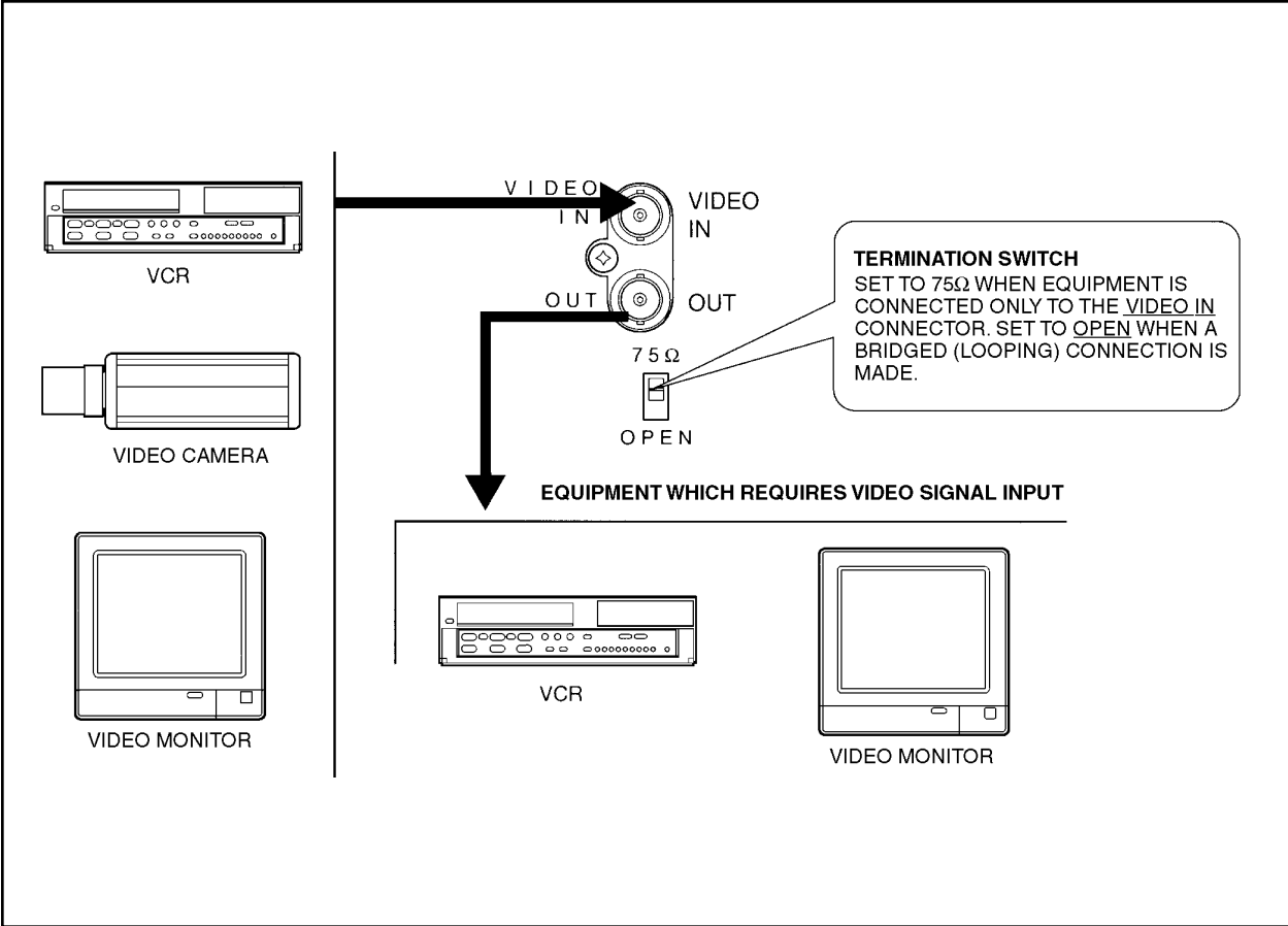
Figure 1. Monitor Connections
